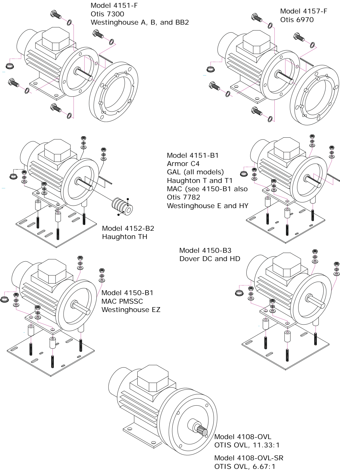
Figure 1. Motor Configurations
